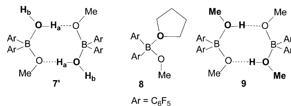
Scheme 3. Adducts of methyl borinate with Lewis bases.
