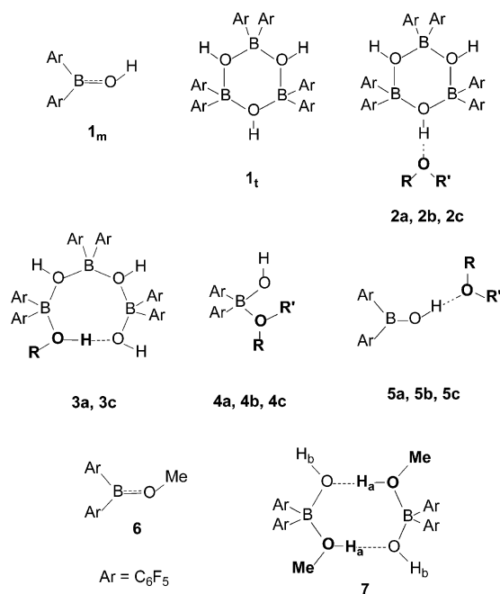
Scheme 1. Monomeric and trimeric borinic acid and their adducts with RR'O bases (a: RR'O = H 2 O, b: RR'O = thf, c: RR'O = MeOH).
