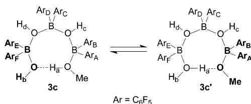
Scheme 5. Proton transfer in oligomer 3c and the resulting interchange of 1 and 6 as chain terminals.
