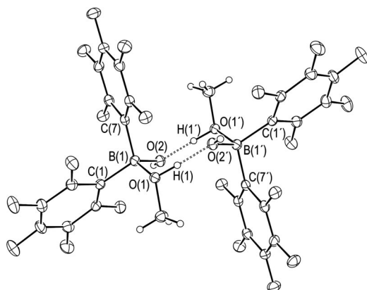
Figure 6. ORTEP drawing of the solid-state structure of the dimeric adduct [\text{Ar}_2\text{B}(\text{OH})(\text{MeOH})]_2 ( 7 ) with a partial labeling scheme. Selected bond lengths [pm] and angles [ ^\circ ]: B(1)–O(1) 154.1(2), B(1)–O(2) 147.2(2), B(1)–C(1) 162.8(3), B(1)–C(7) 163.2(3), O(1)–H(1) 96(3), H(1)···O(2') 153(3), O(1)···O(2') 248.18(18); O(1)–B(1)–O(2) 104.54(14), O(1)–B(1)–C(1) 107.11(13), O(1)–B(1)–C(7) 108.57(14), O(2)–B(1)–C(1) 114.69(15), O(2)–B(1)–C(7) 109.64(14), C(1)–B(1)–C(7) 111.84(14), O(1)–H(1)···O(2') 175(3). Primes address symmetry-equivalent atoms ( 1 - x, -y, 1 - z ).
