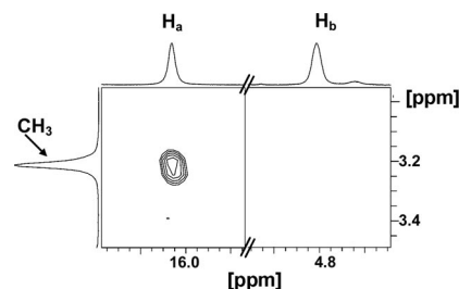
Figure 4. Selected regions of the spectrum of a ^1\text{H} COSY analysis of a \text{CD}_2\text{Cl}_2 solution of 7 (183 K), showing that the Me group has a scalar cross-peak with \text{H}_a only and not with \text{H}_b (Scheme 1). The same experiment does not show a correlation between \text{H}_a and \text{H}_b .
