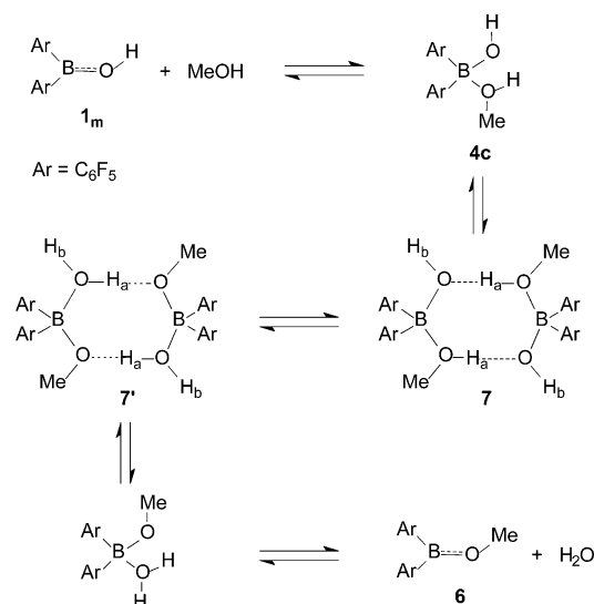
Scheme 4. The esterification–hydrolysis equilibrium.
