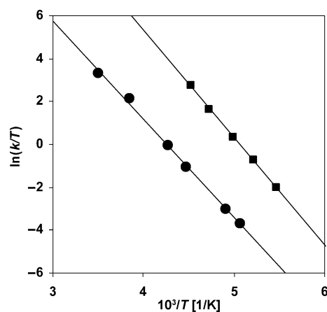
Figure 7. Eyring plot of the kinetic constants for the hindered rotation around the B–OR bond in 1 ( \text{R} = \text{H} , ■) and 6 ( \text{R} = \text{Me} , ●).
