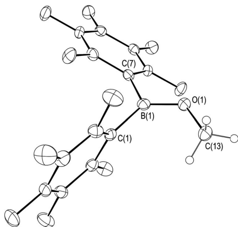
Figure 8. ORTEP drawing of the solid-state structure of the ester [\text{Ar}_2\text{BOMe}] ( 6 ) with a partial labeling scheme. Selected bond lengths [pm] and angles ^\circ : B(1)–O(1) 132.4(3), B(1)–C(1) 158.6(4), B(1)–C(7) 157.4(4), O(1)–C(13) 144.8(3); O(1)–B(1)–C(1) 123.5(2), O(1)–B(1)–C(7) 118.0(2), C(1)–B(1)–C(7) 118.5(2), B(1)–O(1)–C(13) 123.3(2); C(1)–B(1)–O(1)–C(13) 0.8(4), C(1)–B(1)–O(1)–C(13) -177.8(2) .
