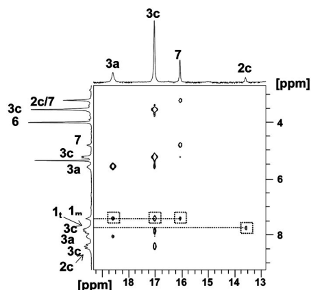
Figure 3. Section of a ^1\text{H} EXSY/NOESY experiment performed with a solution of 1 treated with 0.23 equiv. of MeOH ( \text{CD}_2\text{Cl}_2 , 183 K), showing the intramolecular (NOE) and intermolecular (exchanges shown by dotted squares and straight lines) correlations of the hydrogen-bonded OH protons. The methyl region of the same spectrum shows the exchange between the methoxy group of 6 and the methyl groups of adducts 7 and 3c .
