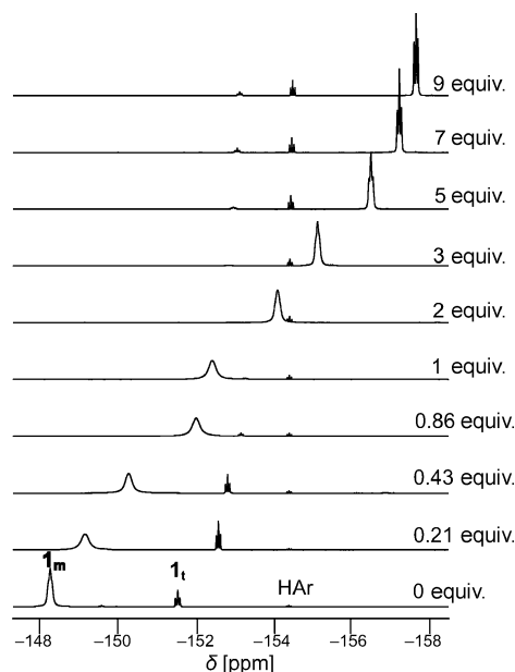
Figure 1. para region of the 19 F NMR spectra of 1 treated with increasing amounts of MeOH (the number of equivalents added is shown for each spectrum) in CD 2 Cl 2 at 283 K. At this temperature, 1 m and 1 t are in fast exchange with their respective adducts with methanol, so that mol-fraction-weighted average resonances are observed. The formation of pentafluorobenzene (labeled as HAr) indicates some progressive decomposition.
