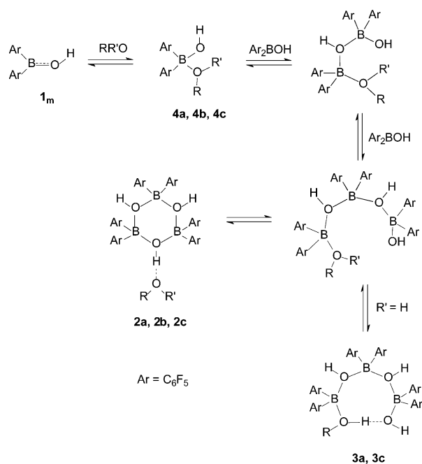
Scheme 2. Oligomerization of 1 in the presence of Lewis bases RR'O.
