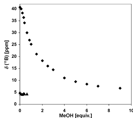
Figure 5. Variation of the chemical shifts of the (averaged) ^{11}\text{B} NMR resonances of the monomeric ( \blacklozenge ) and trimeric ( \blacktriangle ) species, during a titration of 1 with methanol, at 283 K.
